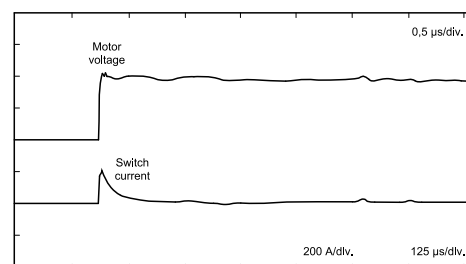
Fig. 6 Clean switch-on of motor
