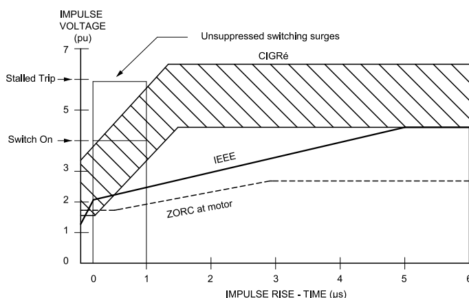
Fig. 4 Impulses withstand levels of medium voltage motors.
