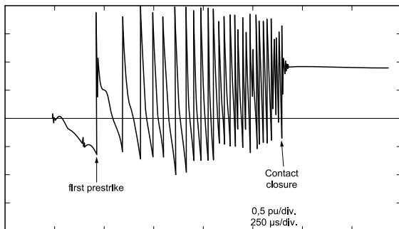
Fig. 1 Multiple pre-striking during routine motor switch-on.
