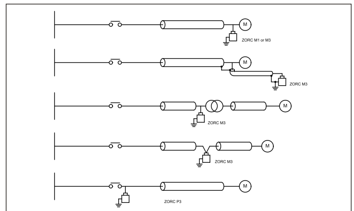
Fig. 8 Preferred connections of ZORC surge suppressors
