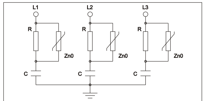
Fig. 5 Patented ZORC circuit and technique.
