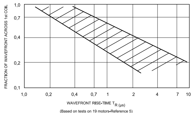
Fig. 3 Percentage of voltage wave-front appearing across line-end coil as a function of rise-time. Ref: Publication 5.
