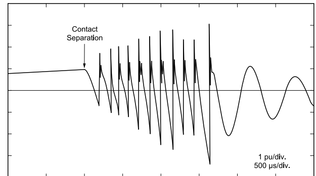
Fig. 2 Multiple re-striking (re-ignition) during interruption of a motor starting current. i.e. Stalled tripping. Without a ZORC surge suppressor fitted. Ref: Publication 1.
