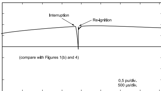
Fig. 7 Single re-strike during interruption of a motor starting current
